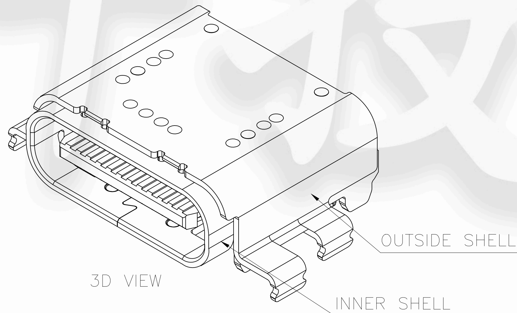
CUSTOMER DRAWING
