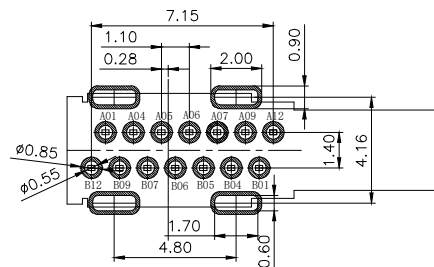
RECOMMENDED P.C.B. LAYOUT TOLERANCE UNSPECIFIED ±0.05mm
